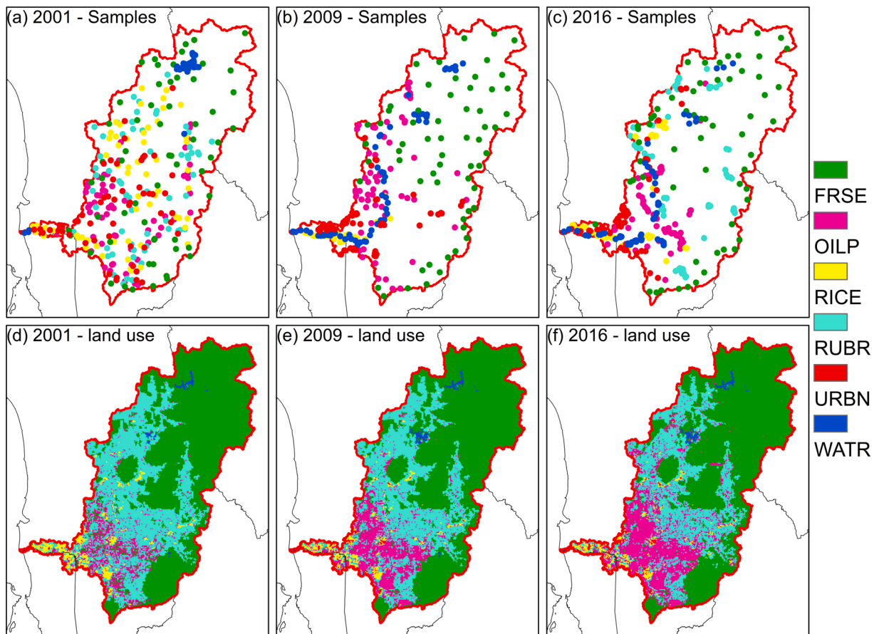
Fig. 4. The locations of the ground samples for (a) 2001, (b) 2009 and (c) 2016 and the spatial distribution of land use land cover of the Muda River Basin in (d) 2001, (e) 2009 and (f) 2016 that was extracted from the improved ESA CCI maps.
