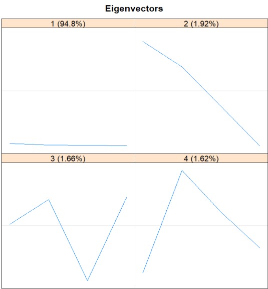
Figure 5: Eigenvector plot obtained by SSA.
