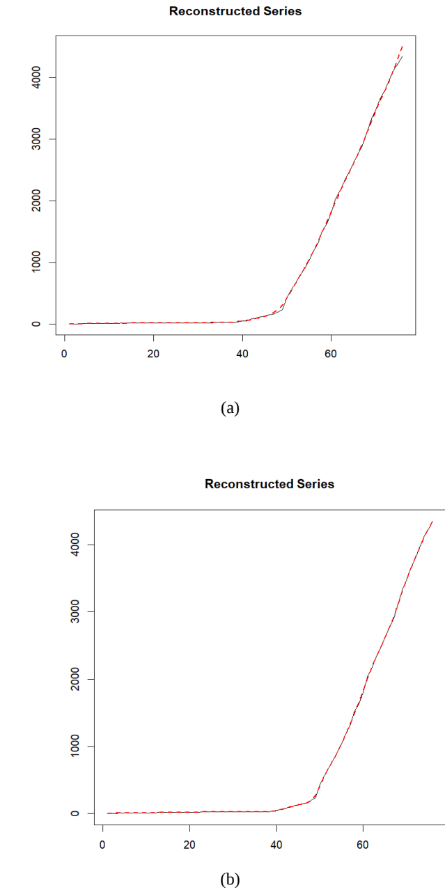
Figure 8: Plot of daily Covid-19 cases reconstructed components from extracted trends using SSA at (a) L=4, ET1 (b) L=4, ET2
