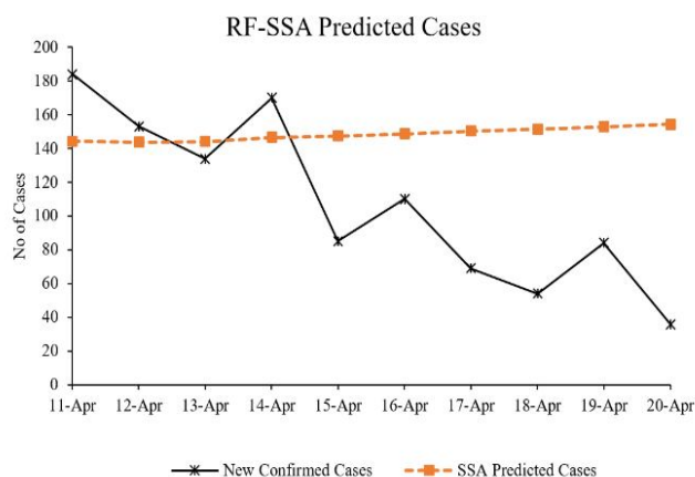
Figure 10: RF-SSA 10-days Ahead vs New Confirmed Cases for Covid-19 in Malaysia
