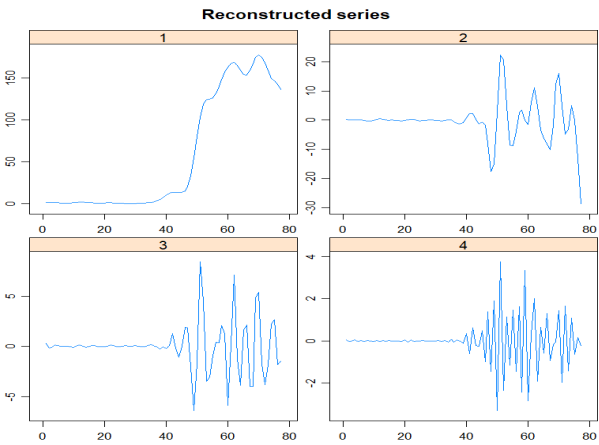
Figure 6: First stage: elementary reconstructed series ( L=4 )
