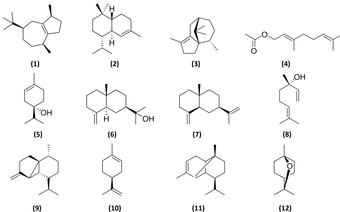
Figure 1. Chemical structures of several major components identified from Goniiothalamus essential oils.
