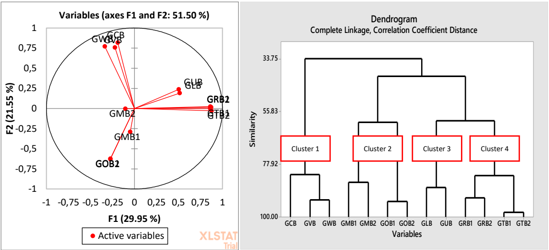
Figure 3. PCA and UPGMA analyses of the composition of Malaysian Goniothalamus leaf oils
